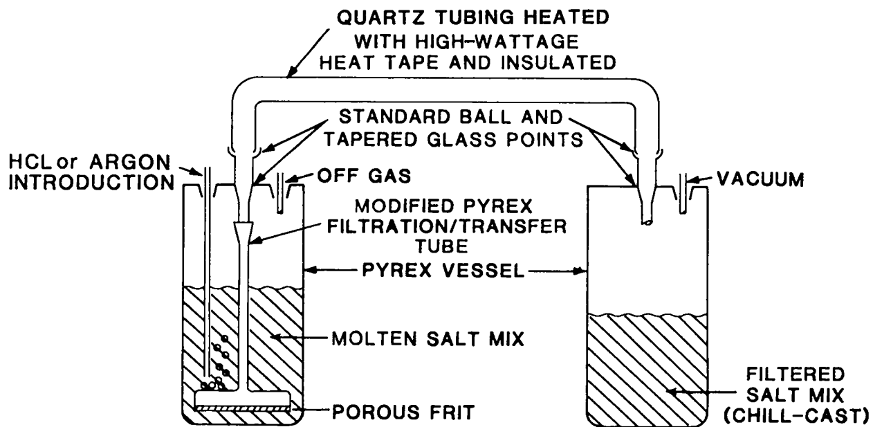
Fig. 8. Apparatus used in semicontinuous pyroredox salt preparation.
