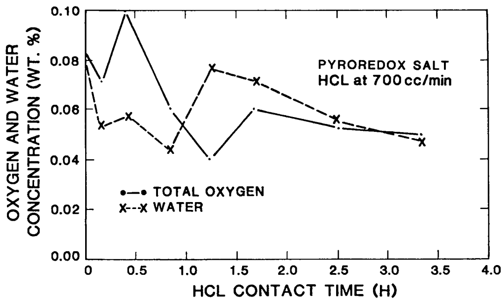
Fig. 4. Total oxygen and water in pyroredox salt as a function of HCl gas contact time.
