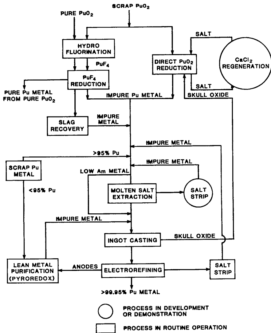
Fig. 1. Plutonium pyrochemical operations at Los Alamos.
