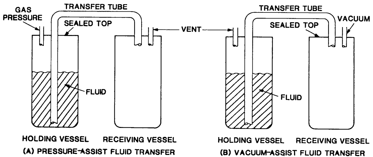
Fig. 7. Schematic of pressure-assist and vacuum-assist fluid transfer.
