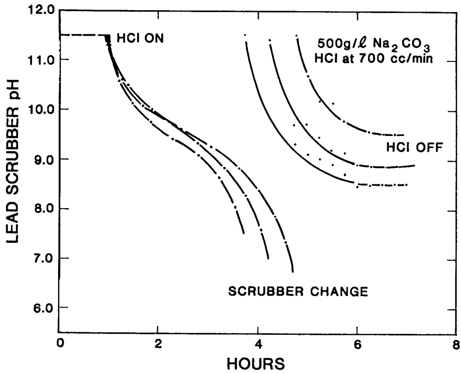
Fig. 6. Neutralization of scrubber solution with anhydrous HCl.
