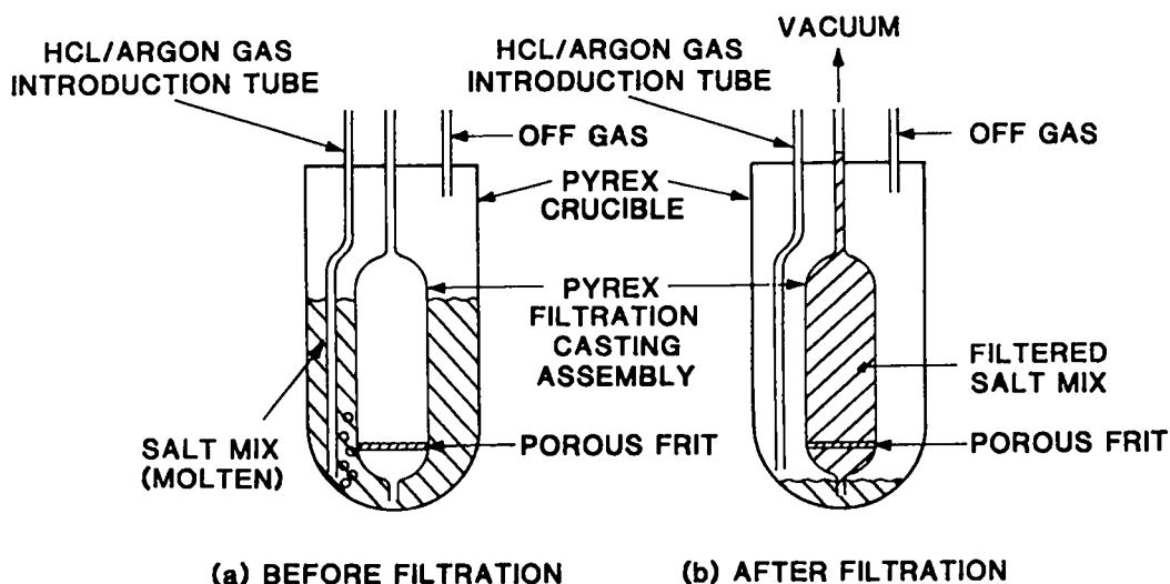
Fig. 2. Batch pyroreodox salt production apparatus.
