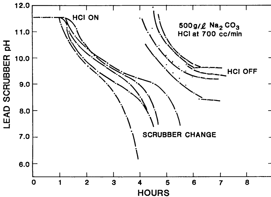
Fig. 5. Neutralization of scrubber solution during pyroredox salt preparation.
